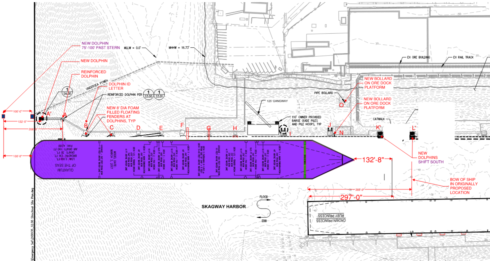
1 STRUCTURAL SITE PLAN SCALE: 1" = 60'
